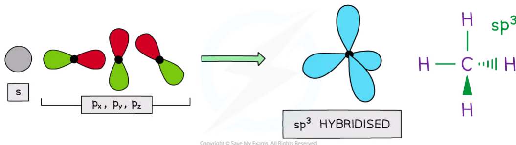
4 x sp^3 hybrid orbitals
