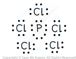
Lewis diagram for \text{PCl}_5
