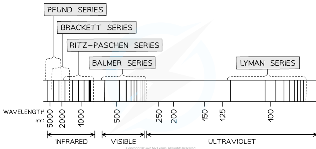
The full hydrogen spectrum
