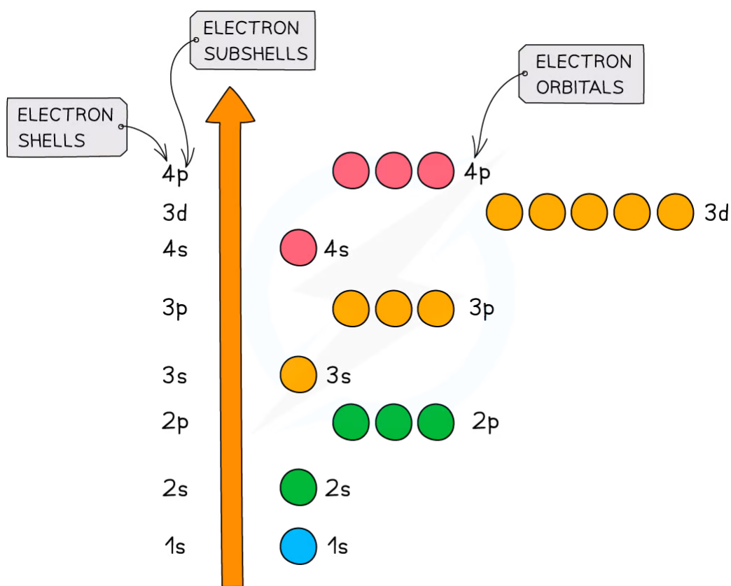
Relative energies of the shells and subshells
